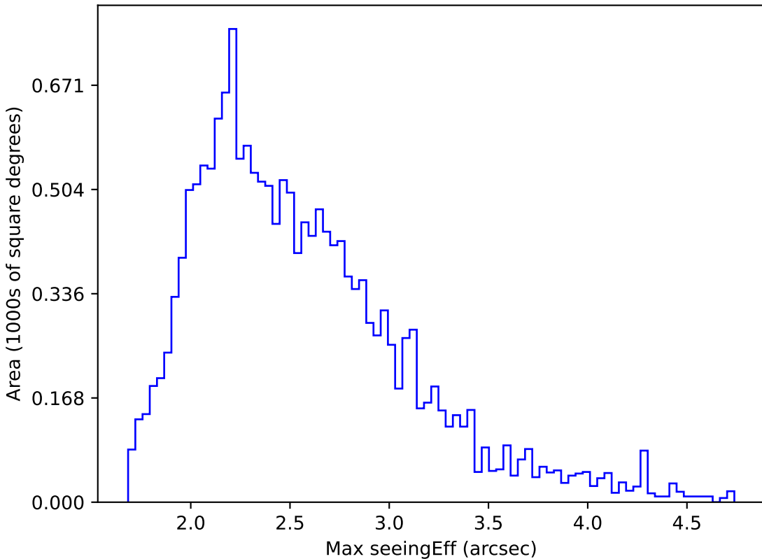
too_elab_r8_d3_gz_v3.4_10yrs WFD z band: Max seeingEff
