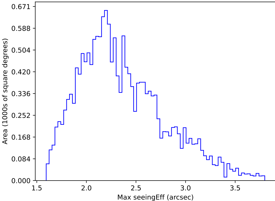
too_elab_r8_d3_gz_v3.4_10yrs WFD y band: Max seeingEff
