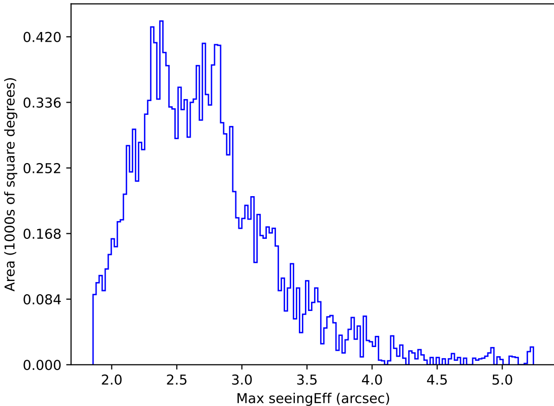
too_elab_r8_d3_gz_v3.4_10yrs WFD r band: Max seeingEff
