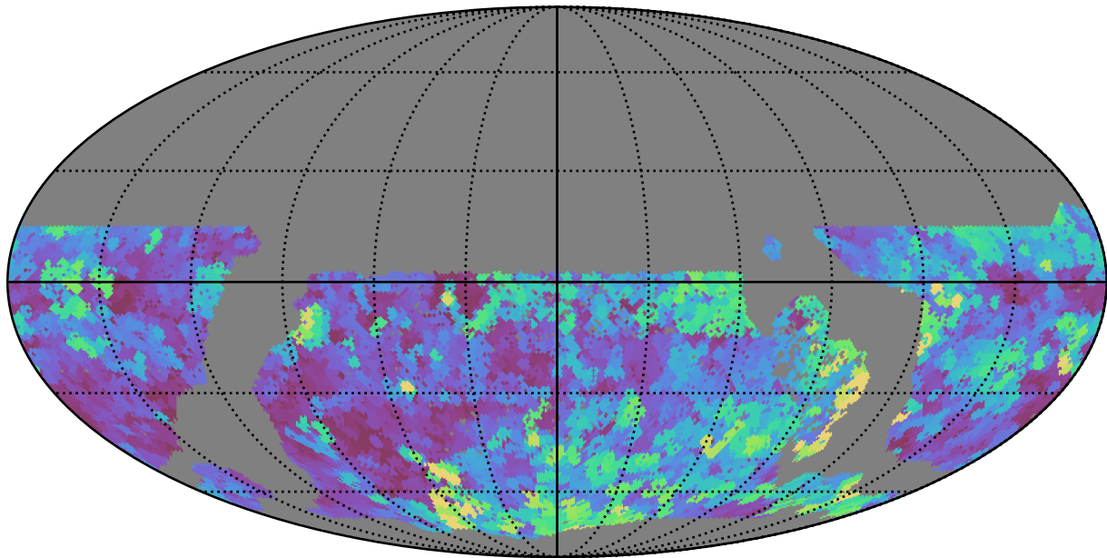
too_elab_r8_d3_gz_v3.4_10yrs WFD g band: Max seeingEff
