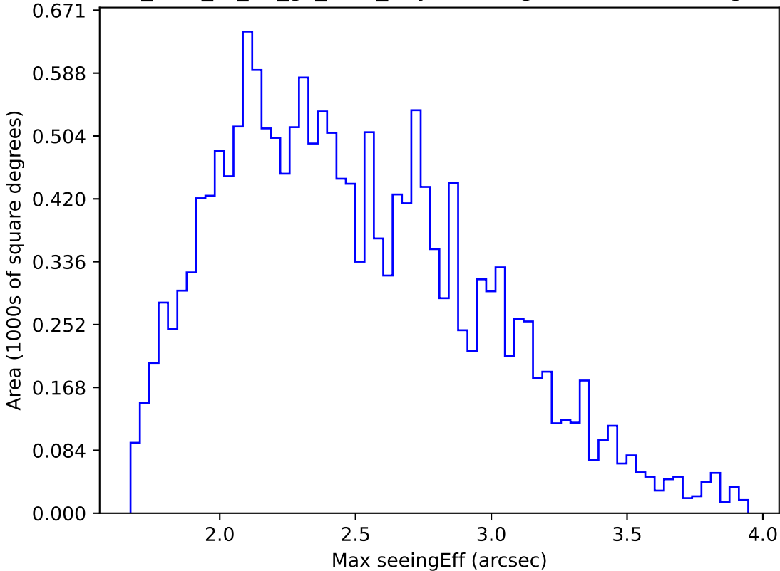
too_elab_r8_d3_gz_v3.4_10yrs WFD g band: Max seeingEff
