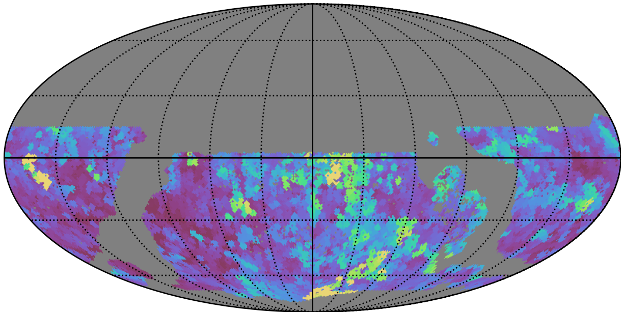
too_elab_r8_d3_gz_v3.4_10yrs WFD all bands: Max seeingEff
