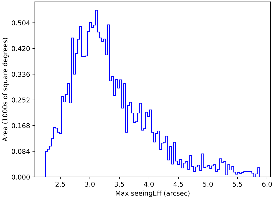
too_elab_r8_d3_gz_v3.4_10yrs WFD all bands: Max seeingEff
