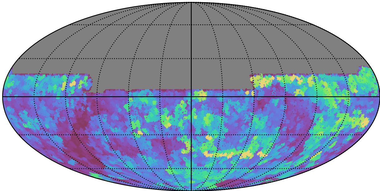
too_elab_r8_d3_gz_v3.4_10yrs All sky y band: Max seeingEff
