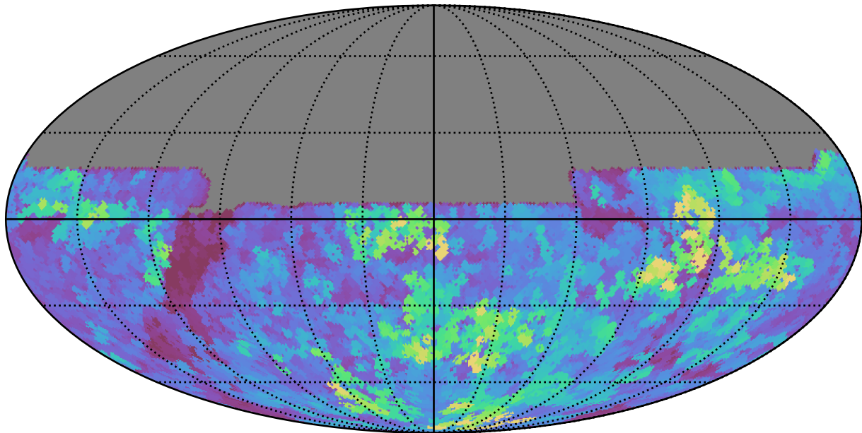
too_elab_r8_d3_gz_v3.4_10yrs All sky u band: Max seeingEff
