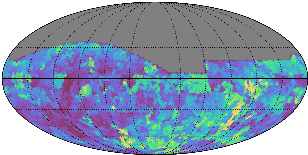
too_elab_r8_d3_gz_v3.4_10yrs All sky g band: Max seeingEff
