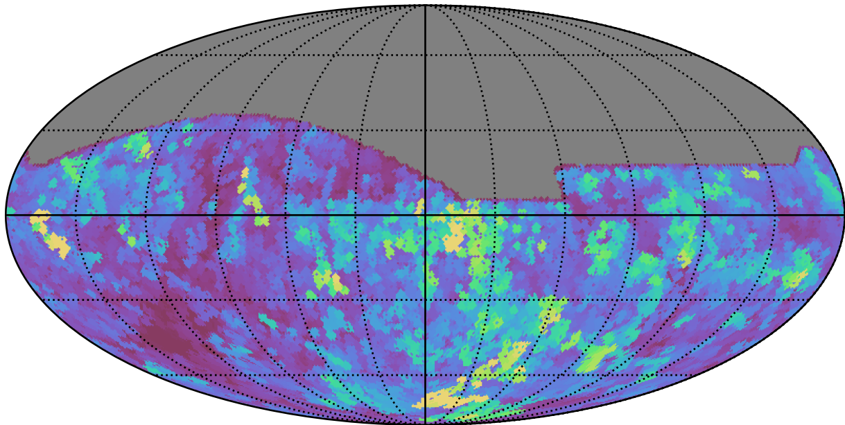
too_elab_r8_d3_gz_v3.4_10yrs All sky all bands: Max seeingEff
