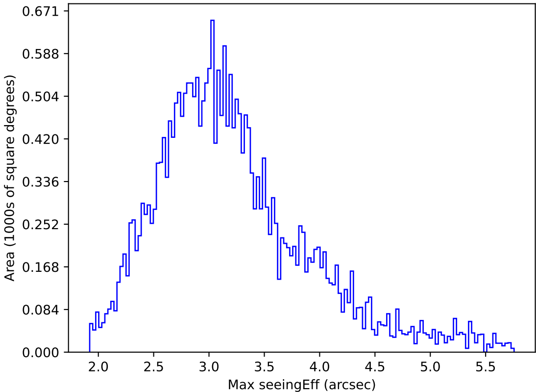
too_elab_r8_d3_gz_v3.4_10yrs All sky all bands: Max seeingEff
