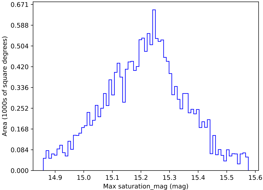
too_elab_r8_d3_gz_v3.4_10yrs WFD z band: Max saturation_mag
