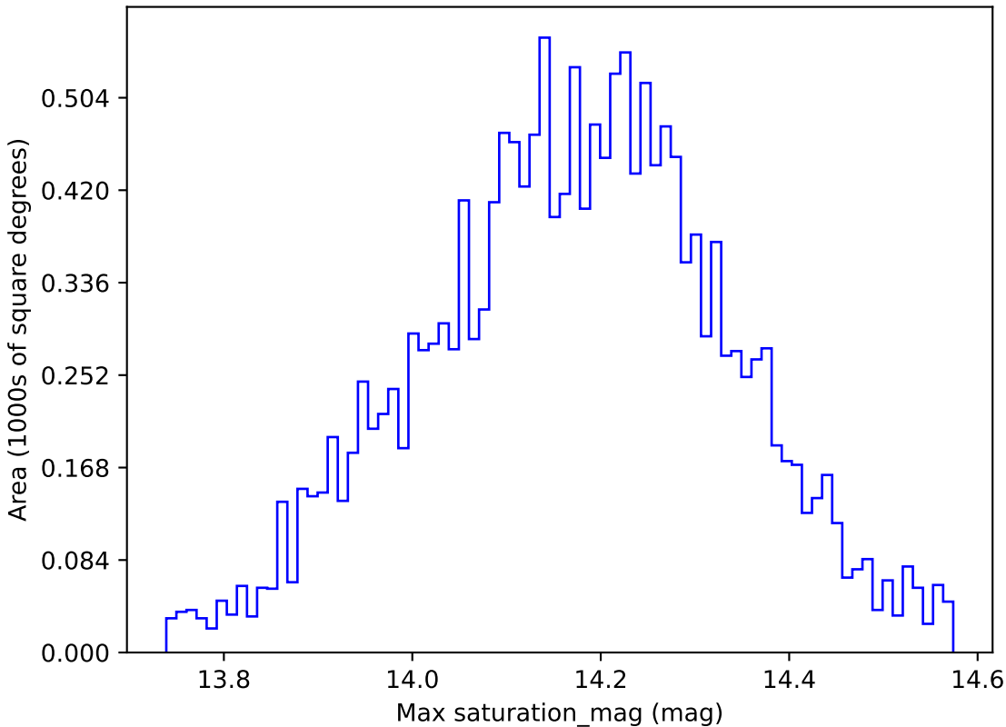
too_elab_r8_d3_gz_v3.4_10yrs WFD y band: Max saturation_mag
