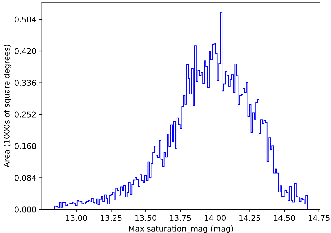
too_elab_r8_d3_gz_v3.4_10yrs All sky u band: Max saturation_mag
