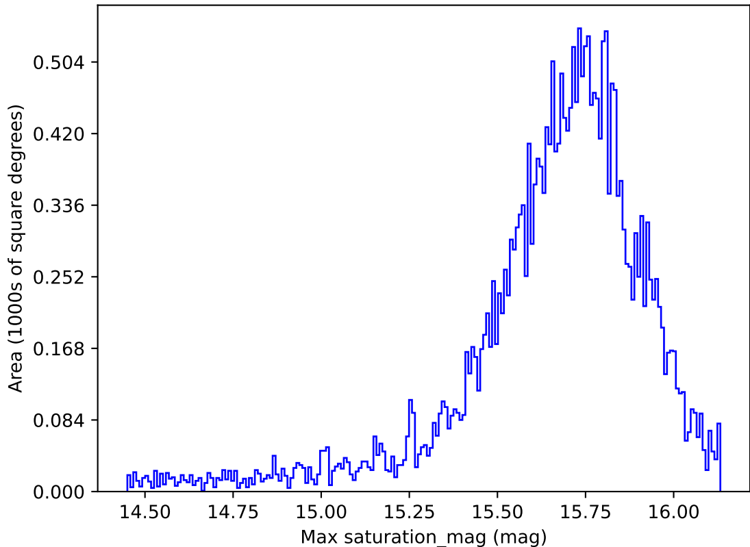
too_elab_r8_d3_gz_v3.4_10yrs All sky r band: Max saturation_mag
