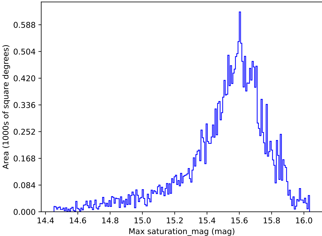
too_elab_r8_d3_gz_v3.4_10yrs All sky i band: Max saturation_mag
