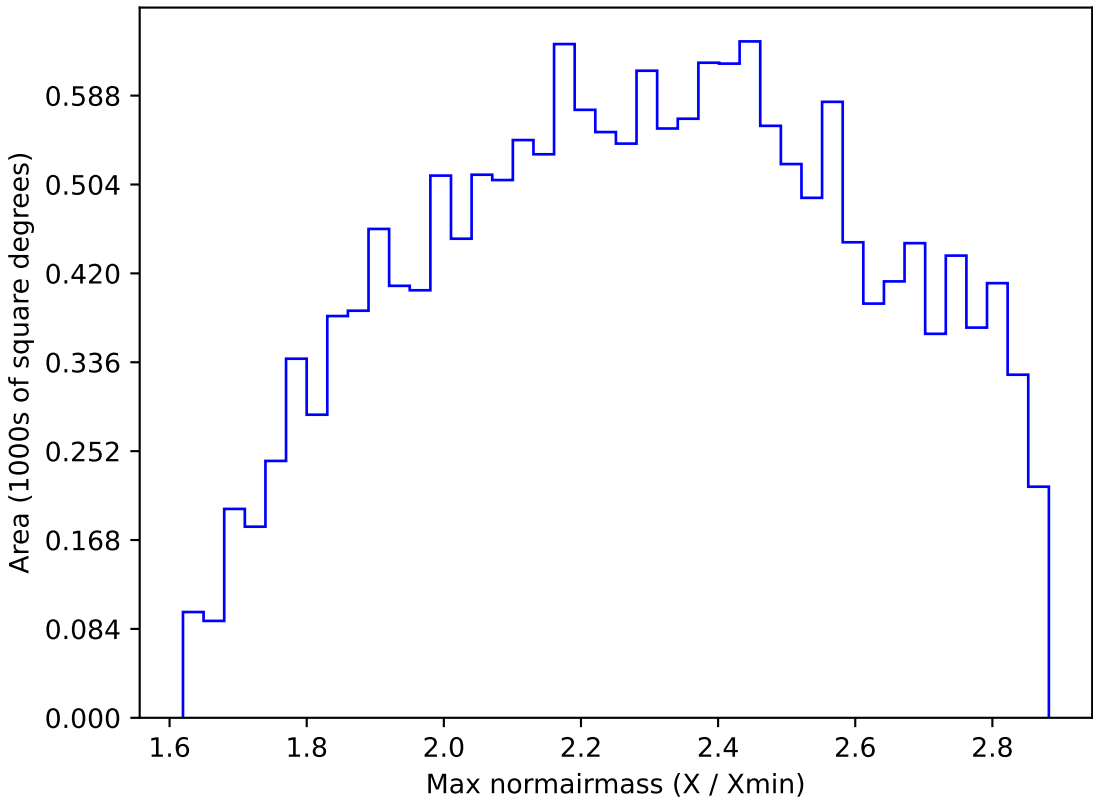
too_elab_r8_d3_gz_v3.4_10yrs WFD z band: Max normairmass
