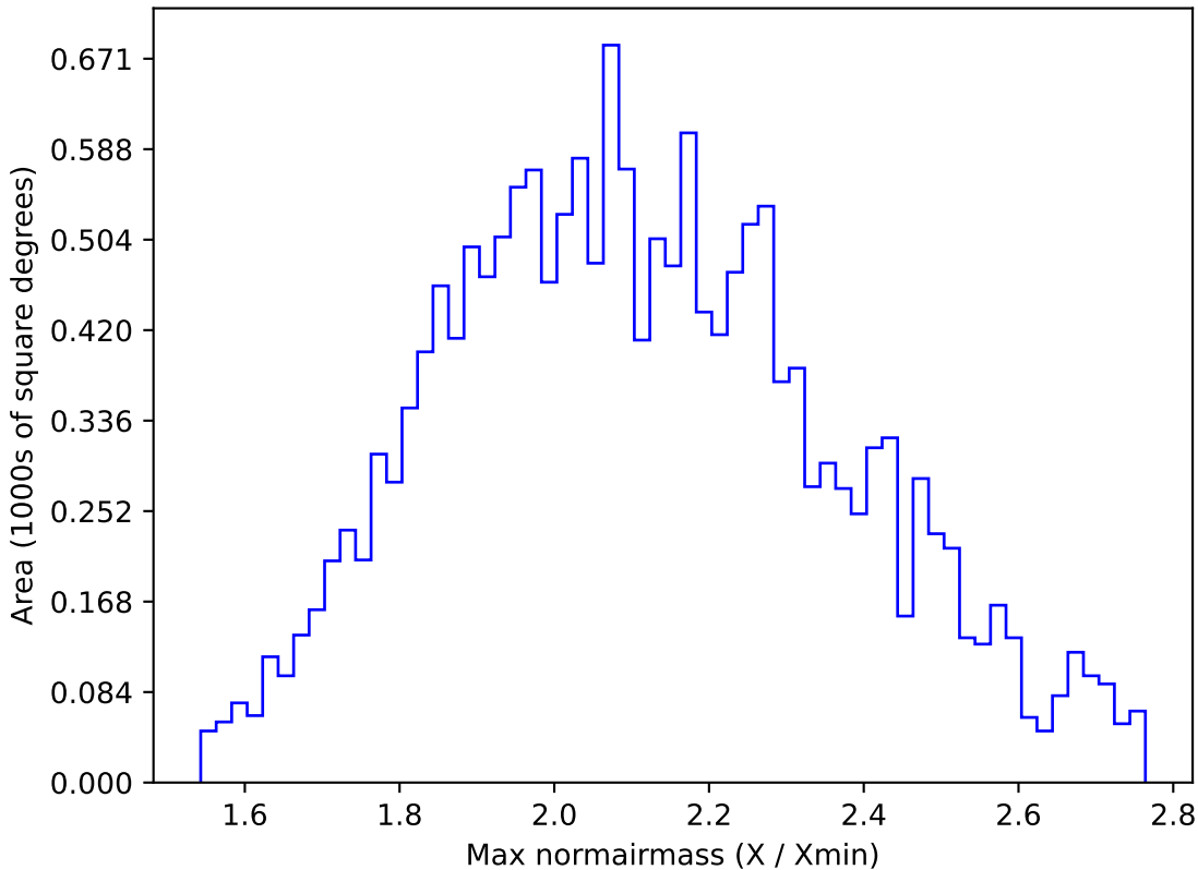
too_elab_r8_d3_gz_v3.4_10yrs WFD y band: Max normairmass
