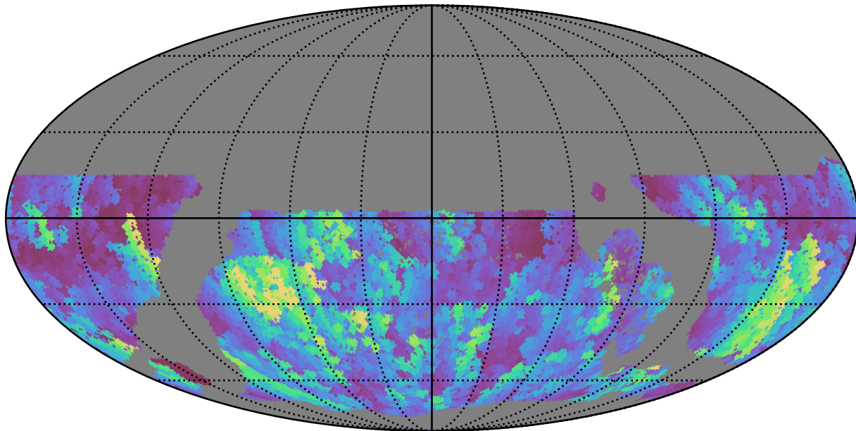
too_elab_r8_d3_gz_v3.4_10yrs WFD u band: Max normairmass
