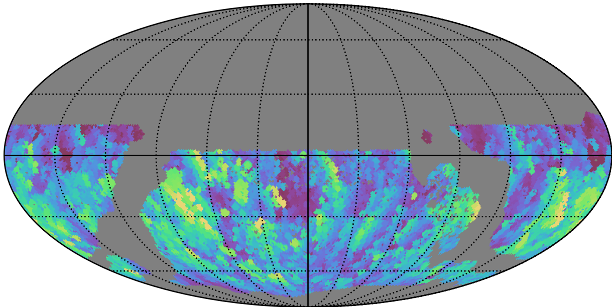
too_elab_r8_d3_gz_v3.4_10yrs WFD g band: Max normairmass
