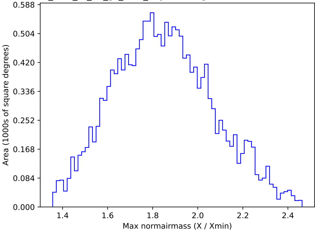
too_elab_r8_d3_gz_v3.4_10yrs WFD g band: Max normairmass
