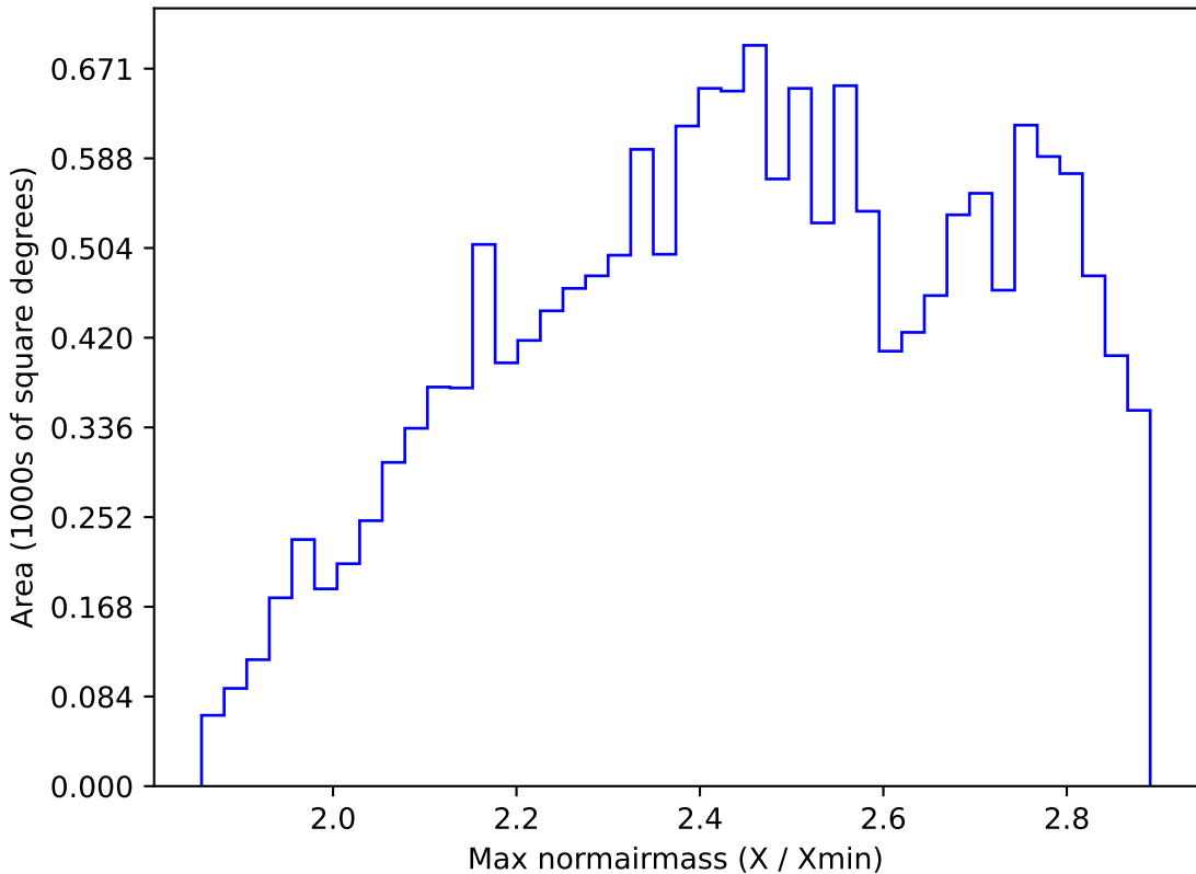
too_elab_r8_d3_gz_v3.4_10yrs WFD all bands: Max normairmass
