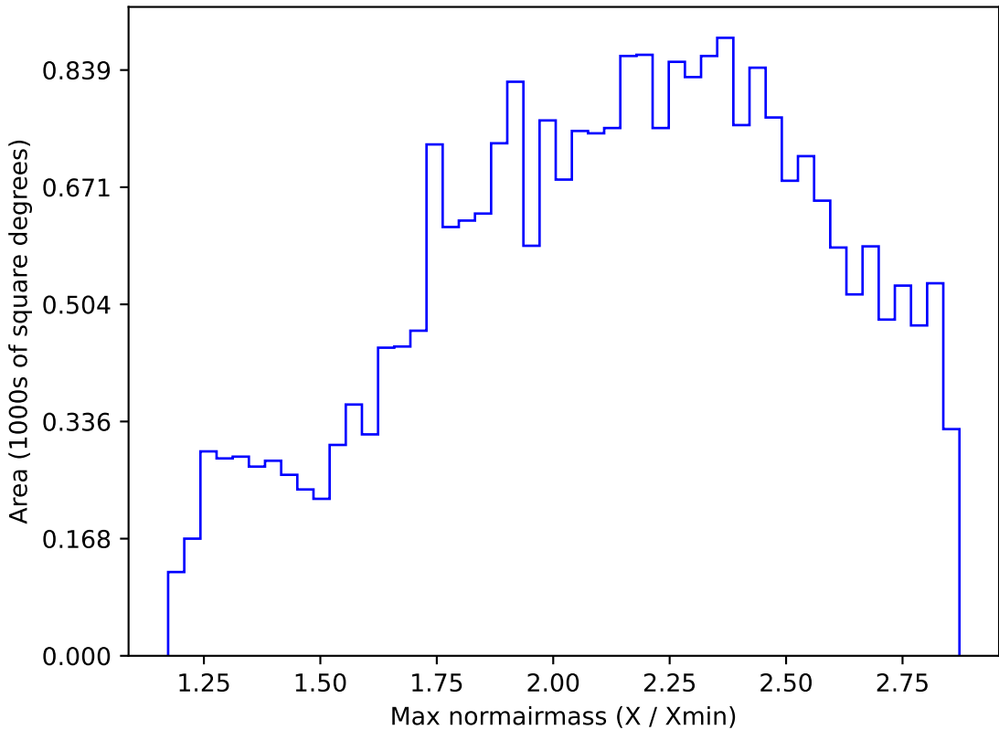
too_elab_r8_d3_gz_v3.4_10yrs All sky z band: Max normairmass
