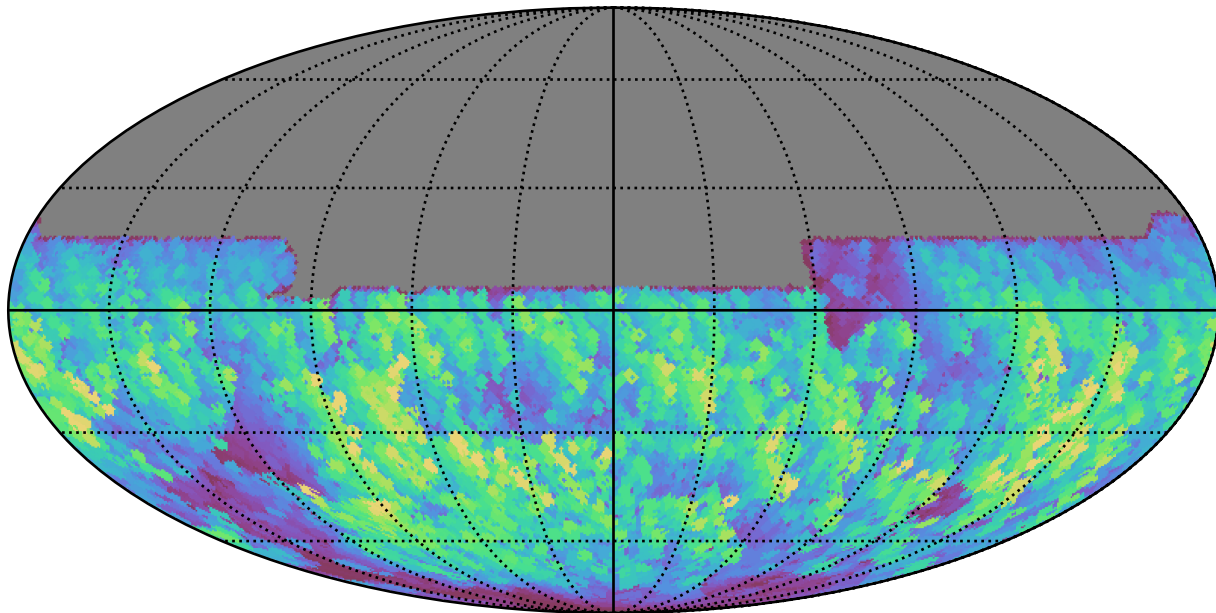
too_elab_r8_d3_gz_v3.4_10yrs All sky y band: Max normairmass
