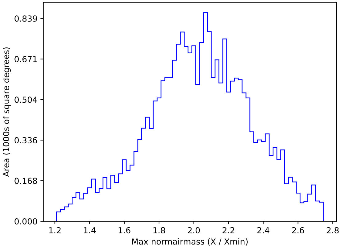
too_elab_r8_d3_gz_v3.4_10yrs All sky y band: Max normairmass
