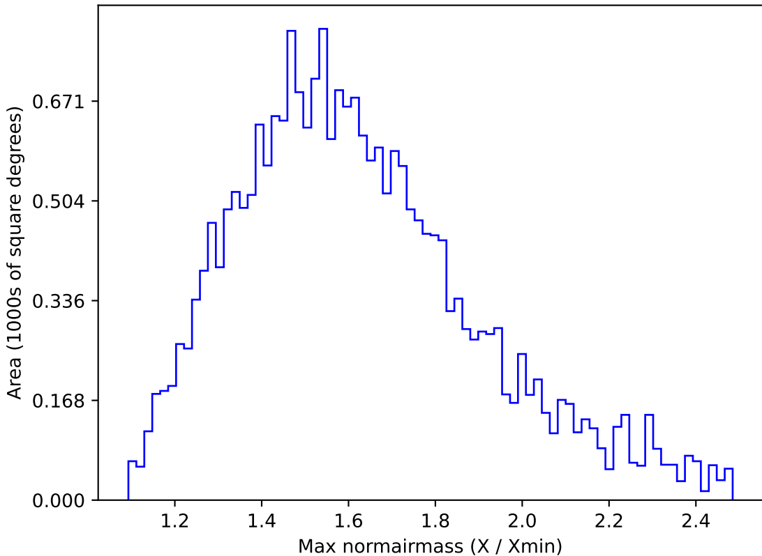
too_elab_r8_d3_gz_v3.4_10yrs All sky u band: Max normairmass
