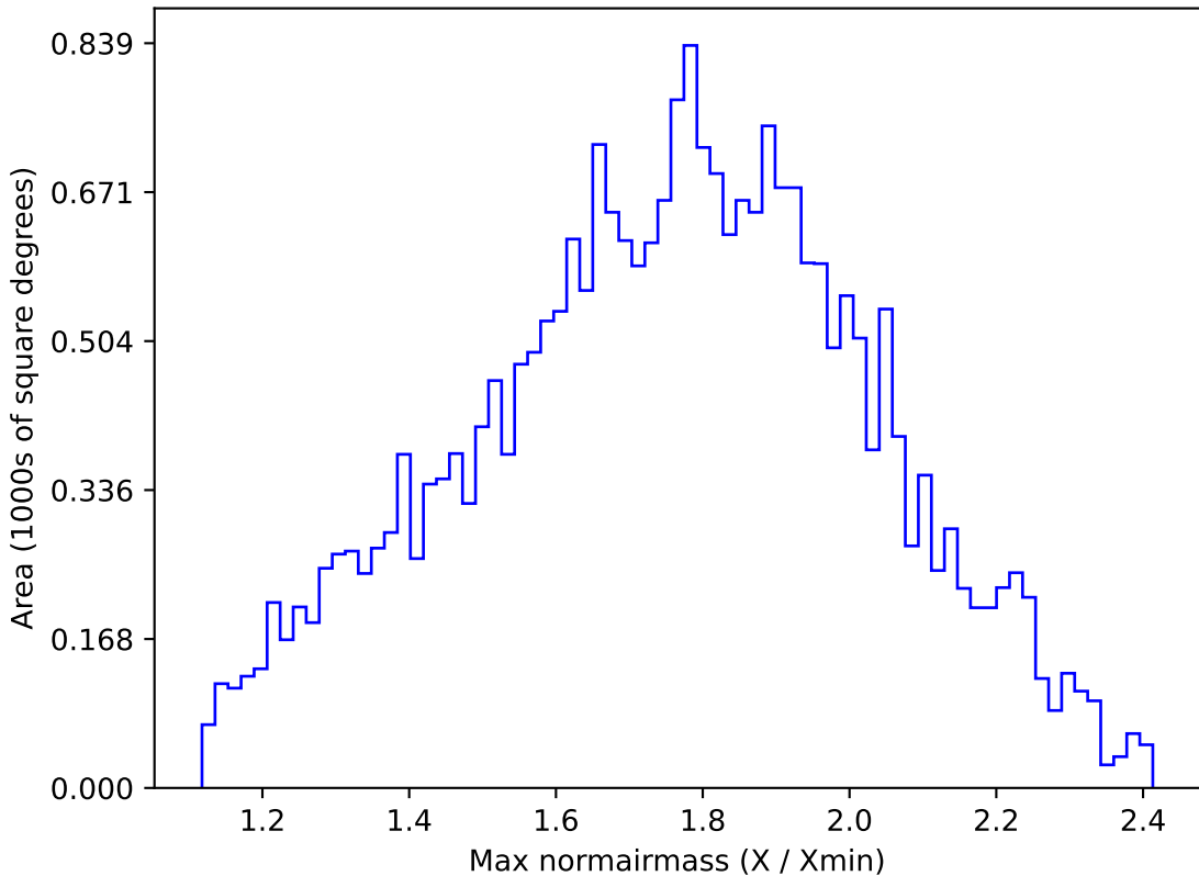
too_elab_r8_d3_gz_v3.4_10yrs All sky g band: Max normairmass
