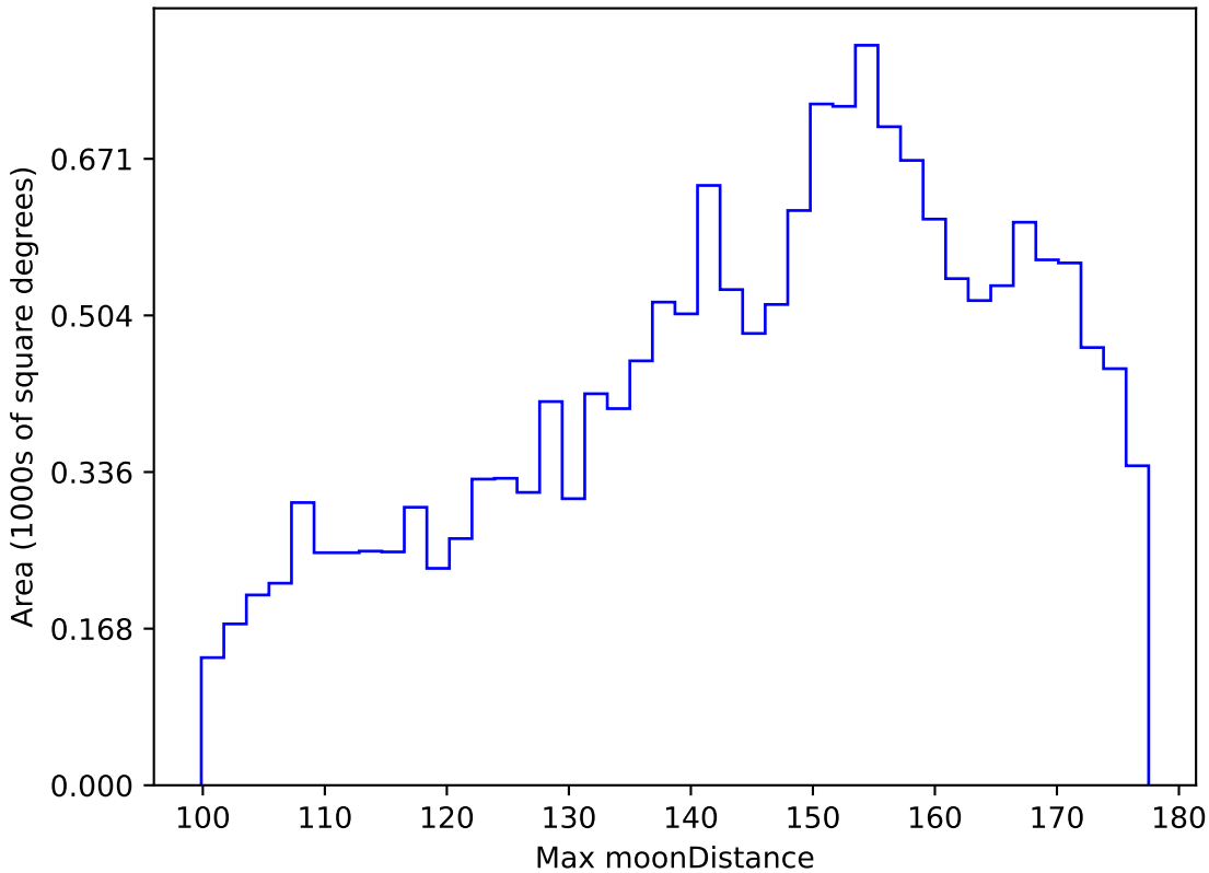
too_elab_r8_d3_gz_v3.4_10yrs WFD y band: Max moonDistance
