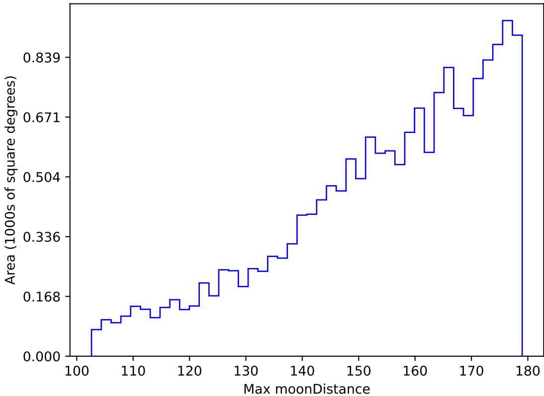
too_elab_r8_d3_gz_v3.4_10yrs WFD u band: Max moonDistance
