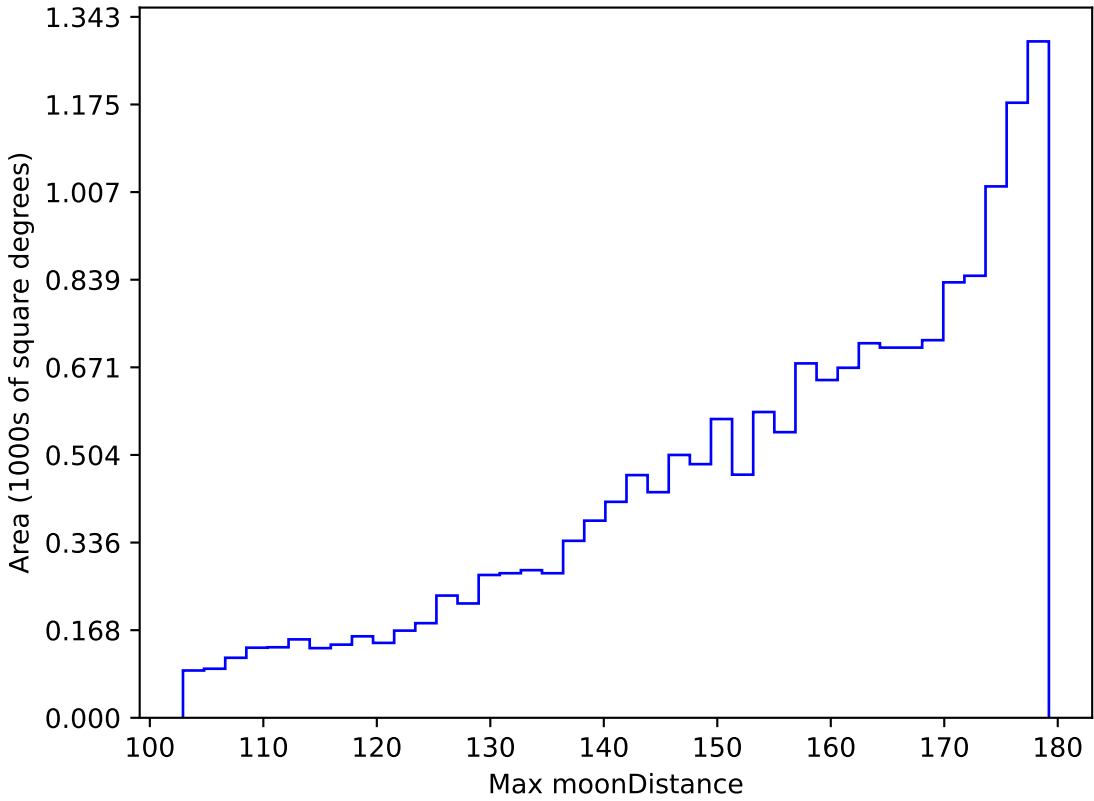
too_elab_r8_d3_gz_v3.4_10yrs WFD i band: Max moonDistance
