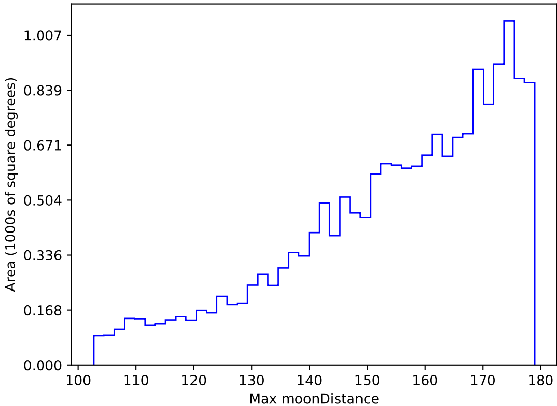
too_elab_r8_d3_gz_v3.4_10yrs WFD g band: Max moonDistance
