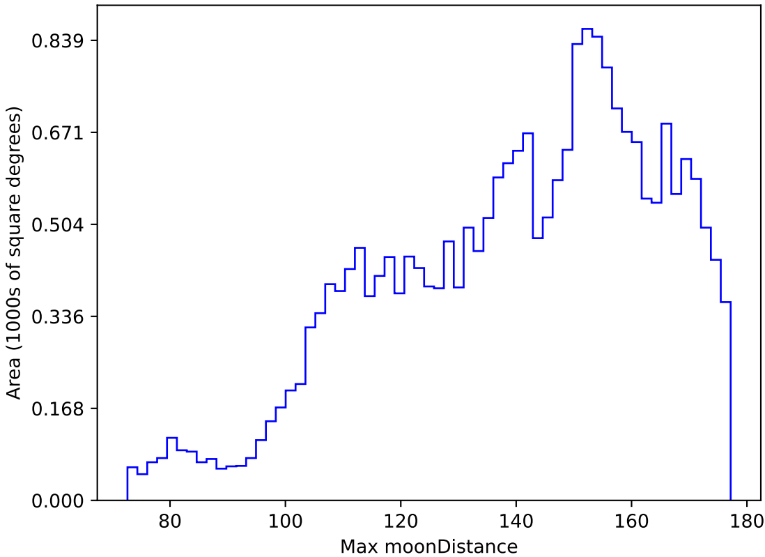
too_elab_r8_d3_gz_v3.4_10yrs All sky y band: Max moonDistance
