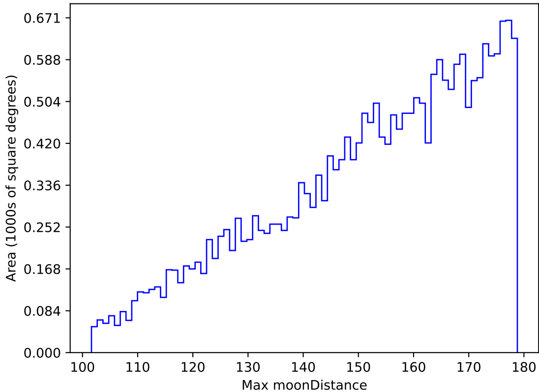
too_elab_r8_d3_gz_v3.4_10yrs All sky u band: Max moonDistance
