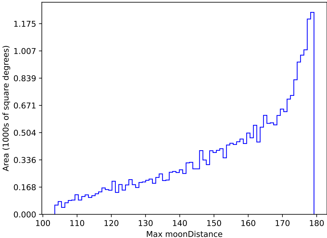
too_elab_r8_d3_gz_v3.4_10yrs All sky r band: Max moonDistance
