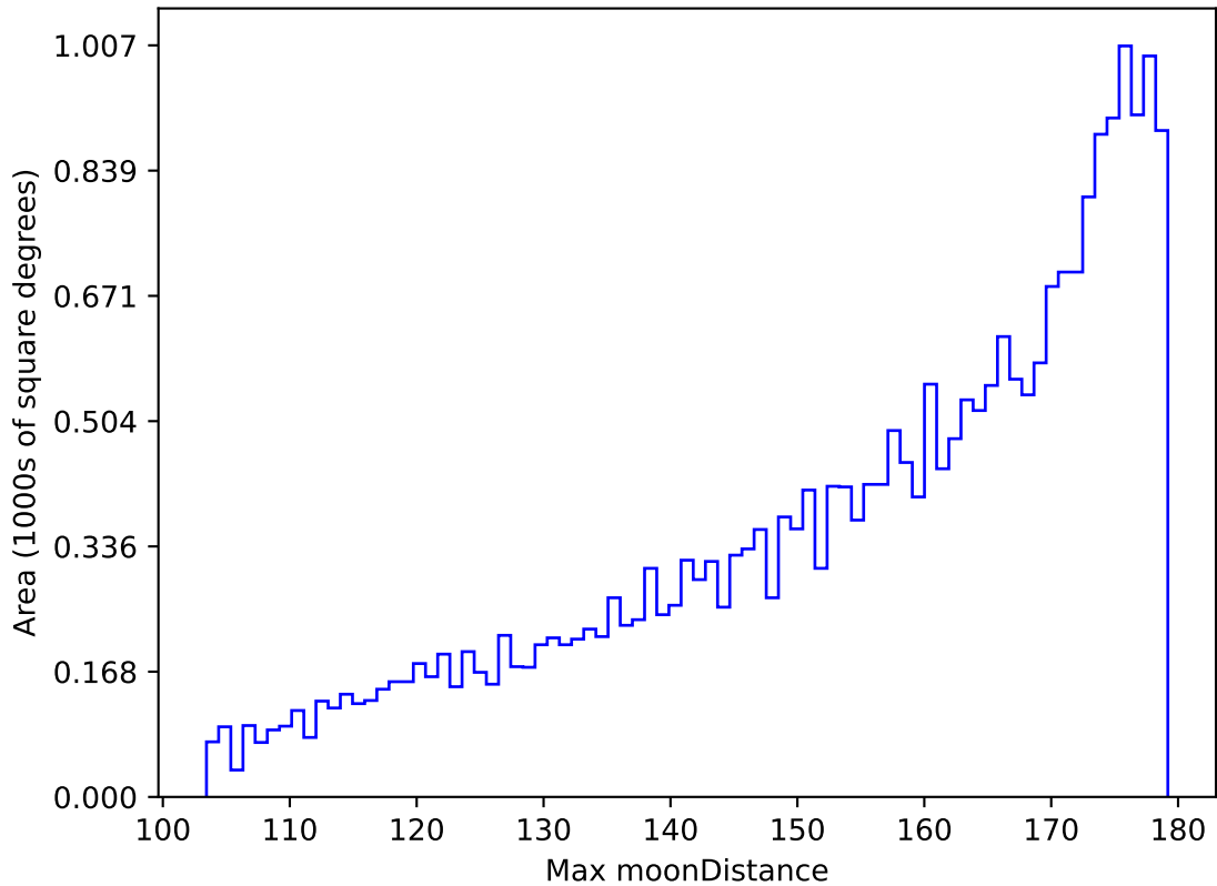
too_elab_r8_d3_gz_v3.4_10yrs All sky i band: Max moonDistance
