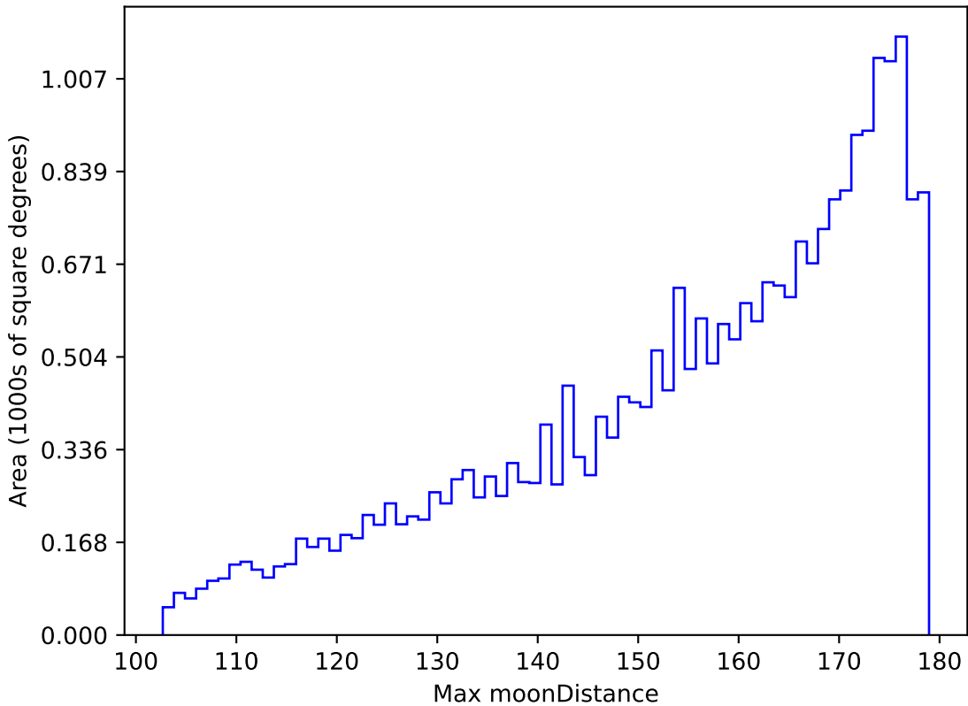
too_elab_r8_d3_gz_v3.4_10yrs All sky g band: Max moonDistance
