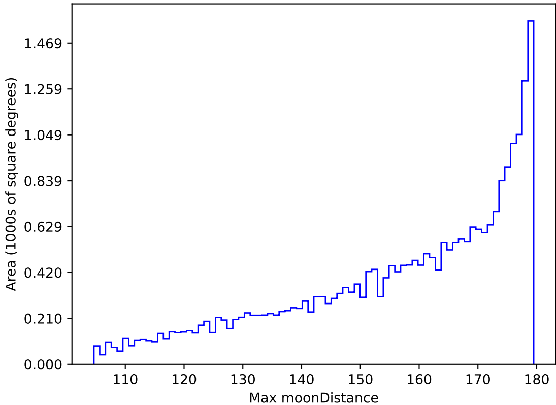
too_elab_r8_d3_gz_v3.4_10yrs All sky all bands: Max moonDistance
