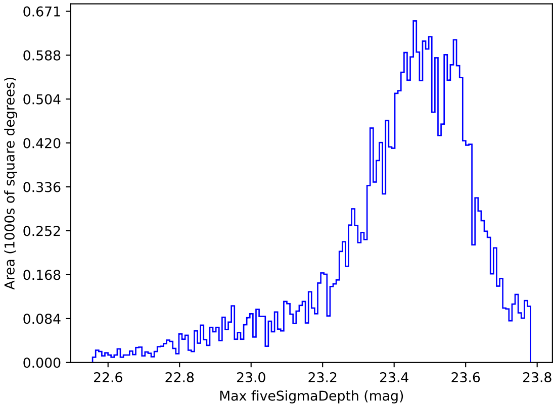
too_elab_r8_d3_gz_v3.4_10yrs Yr 1 z band: Max fiveSigmaDepth
