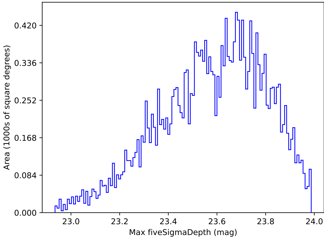
too_elab_r8_d3_gz_v3.4_10yrs Yr 1 u band: Max fiveSigmaDepth
