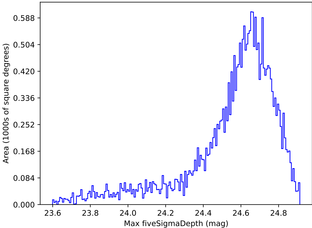
too_elab_r8_d3_gz_v3.4_10yrs Yr 1 r band: Max fiveSigmaDepth
