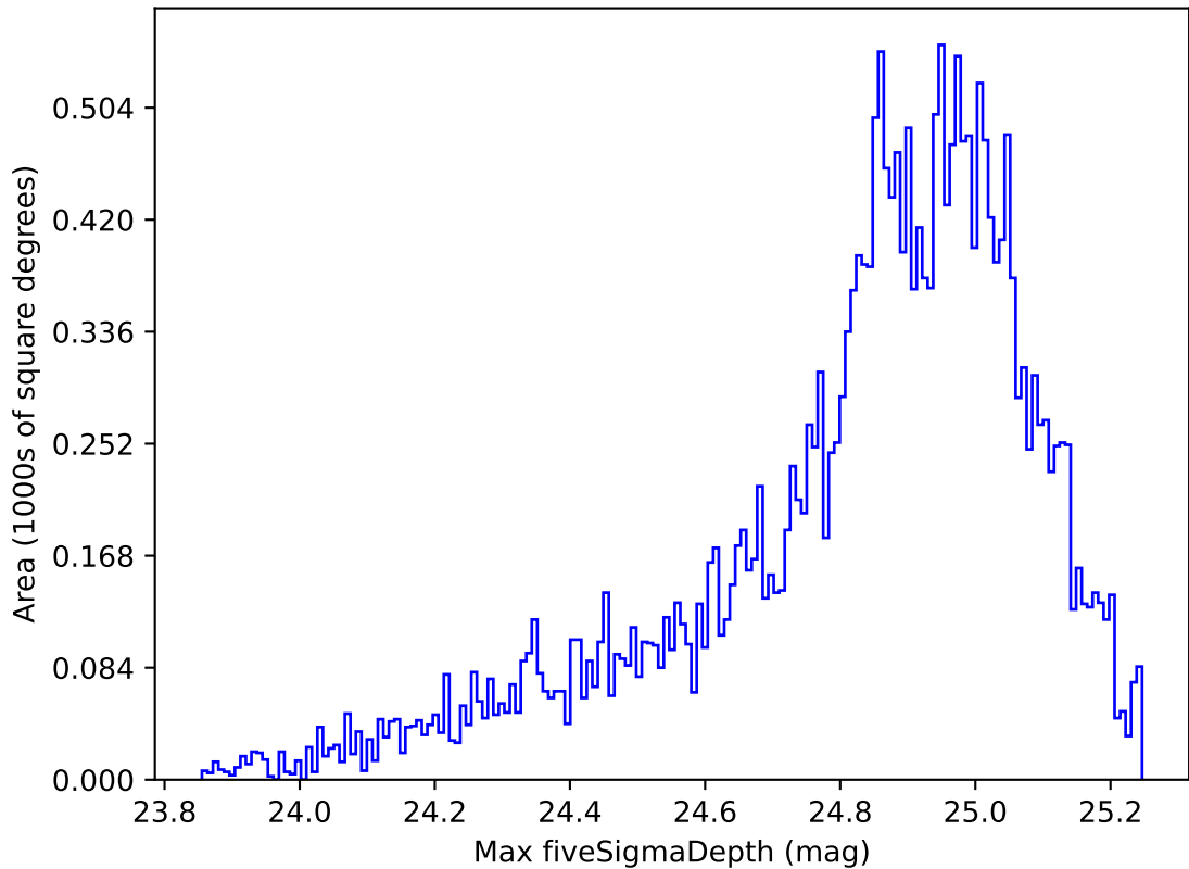
too_elab_r8_d3_gz_v3.4_10yrs Yr 1 g band: Max fiveSigmaDepth
