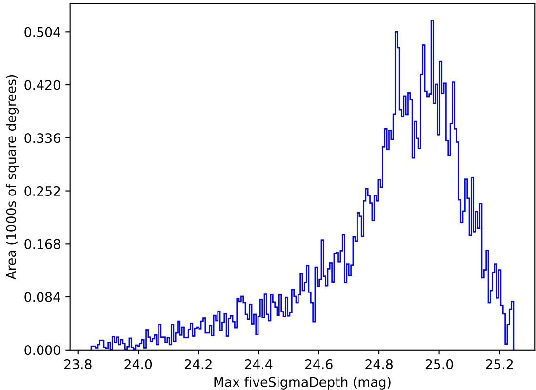
too_elab_r8_d3_gz_v3.4_10yrs Yr 1 all bands: Max fiveSigmaDepth
