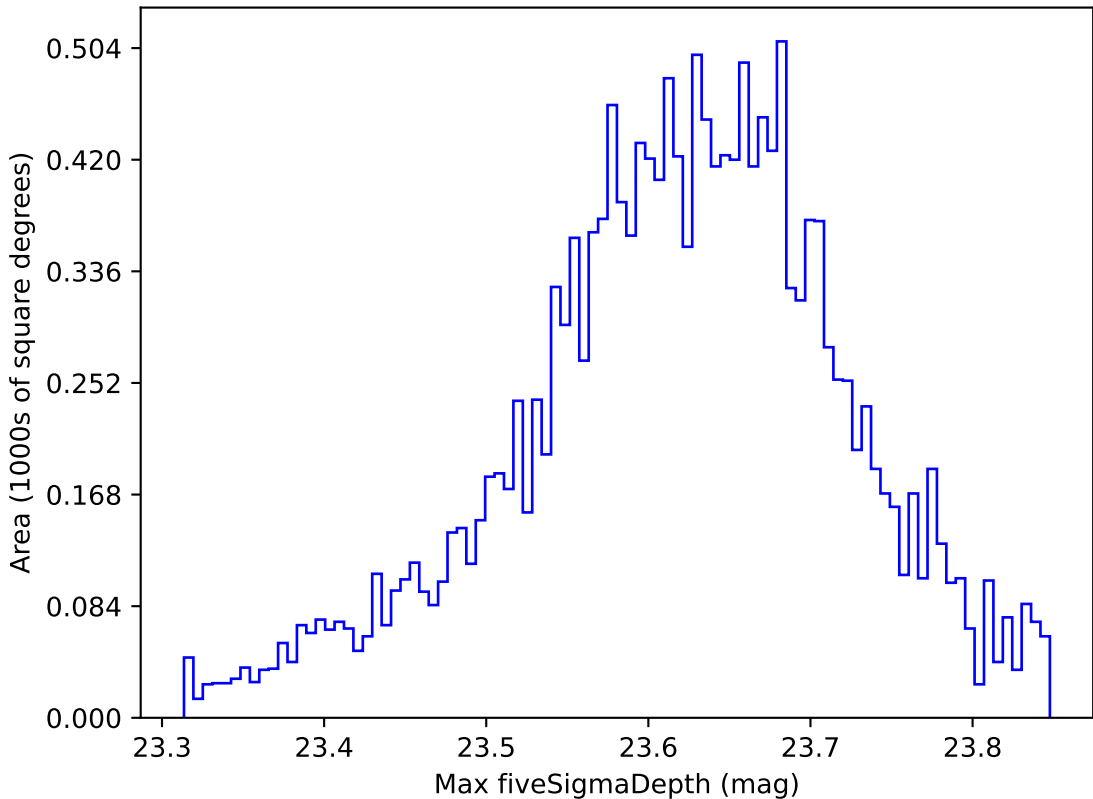
too_elab_r8_d3_gz_v3.4_10yrs WFD z band: Max fiveSigmaDepth
