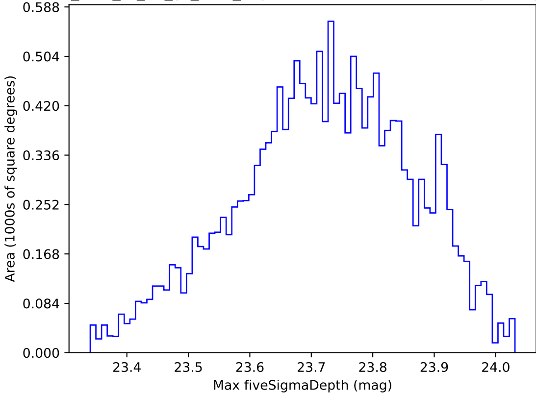
too_elab_r8_d3_gz_v3.4_10yrs WFD u band: Max fiveSigmaDepth
