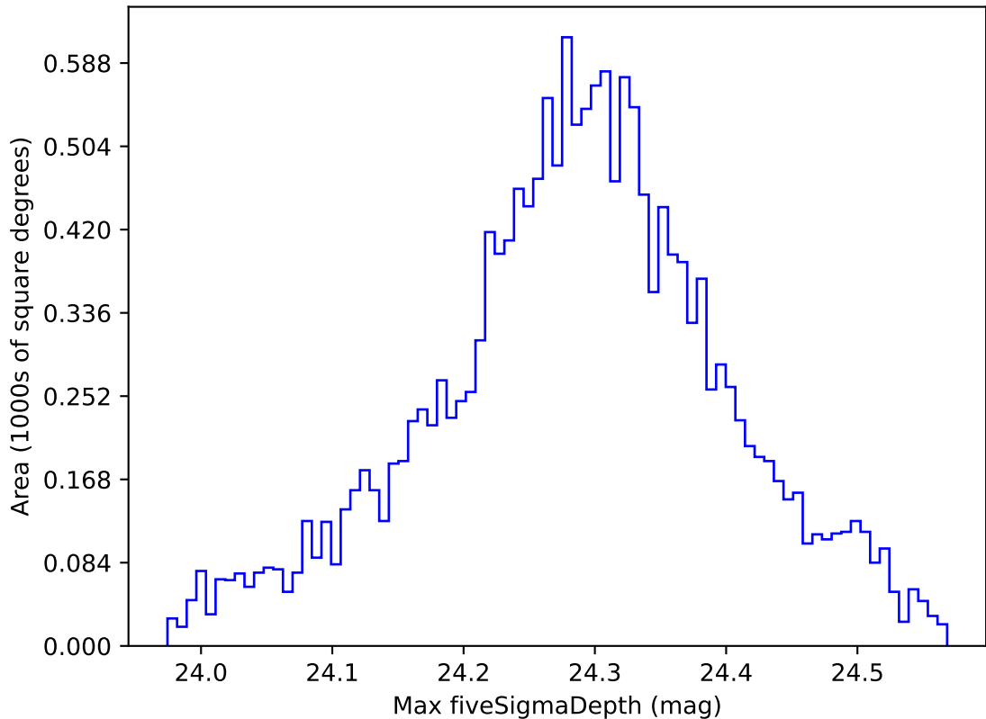
too_elab_r8_d3_gz_v3.4_10yrs WFD i band: Max fiveSigmaDepth
