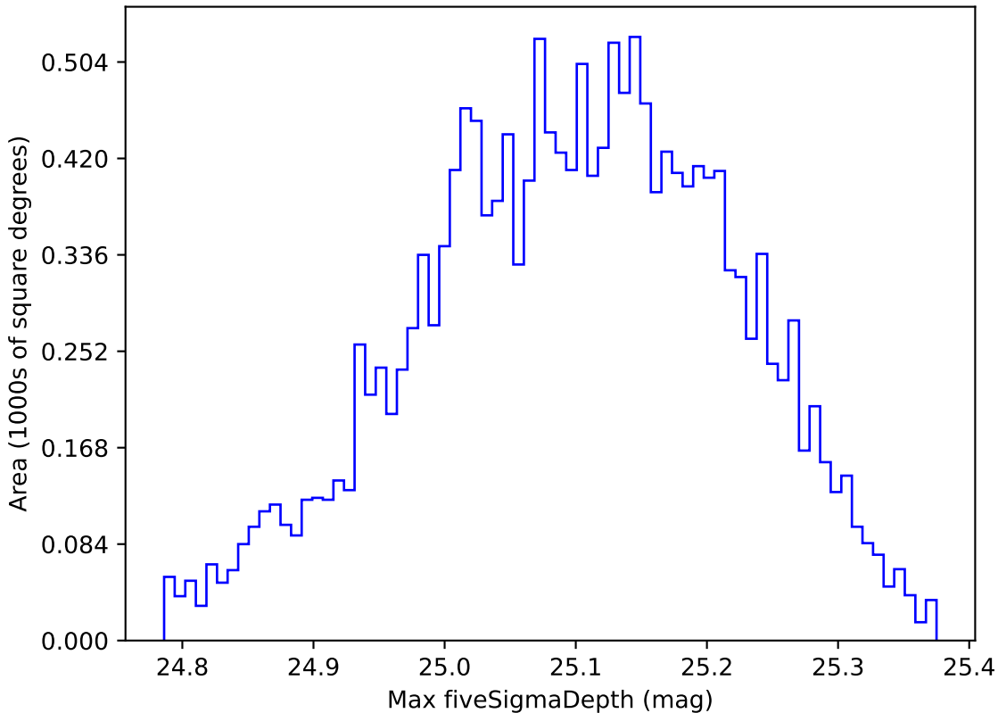
too_elab_r8_d3_gz_v3.4_10yrs WFD g band: Max fiveSigmaDepth
