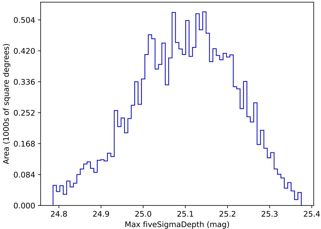
too_elab_r8_d3_gz_v3.4_10yrs WFD all bands: Max fiveSigmaDepth
