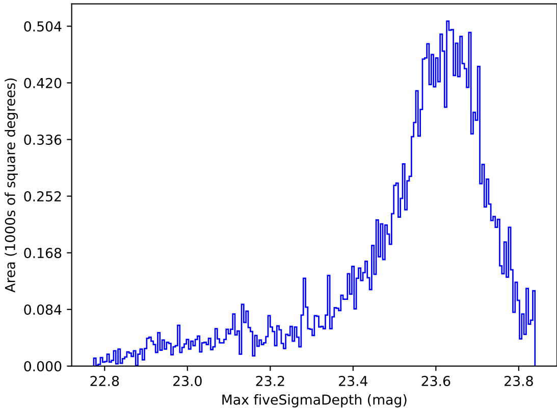
too_elab_r8_d3_gz_v3.4_10yrs All sky z band: Max fiveSigmaDepth
