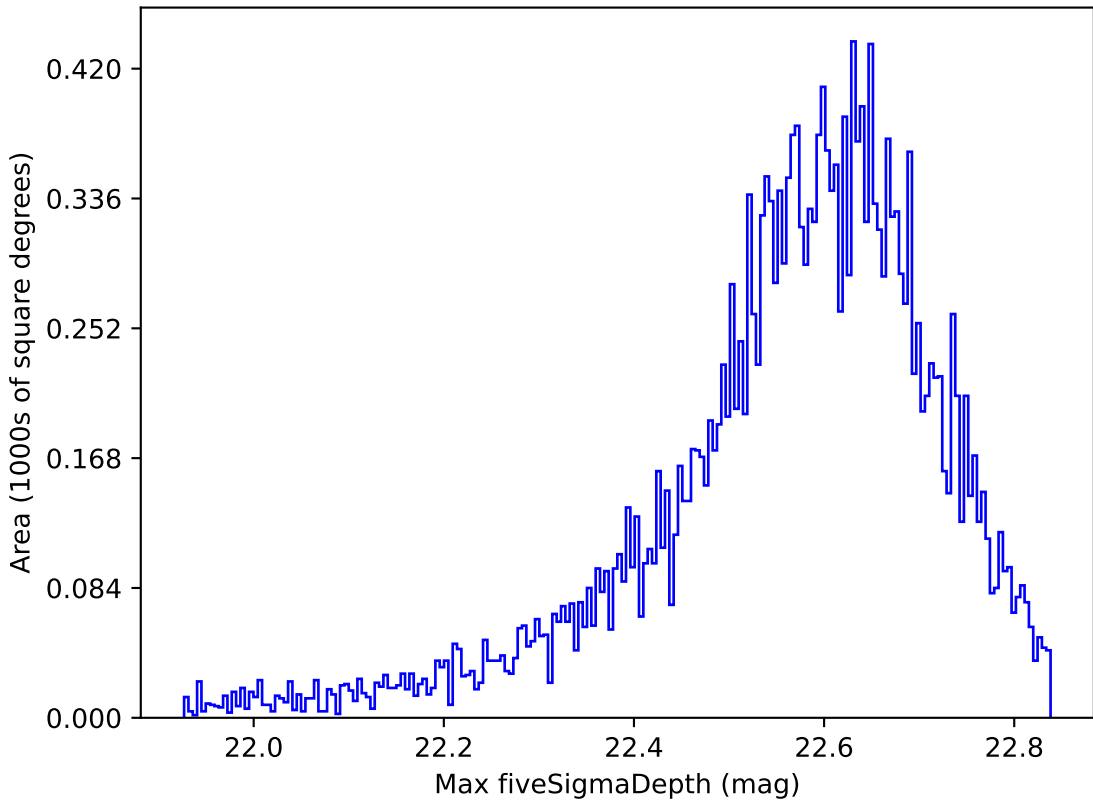
too_elab_r8_d3_gz_v3.4_10yrs All sky y band: Max fiveSigmaDepth
